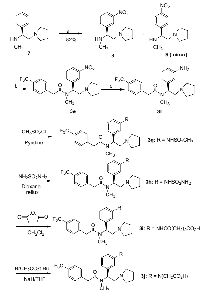
Scheme 2. Reagents and conditions: (a) HNO 3 /H 2 SO 4 ; (b) 4-trifluoromethylphenylacetic acid, DCC/HOBT; (c) Raney Ni, hydrazine, EtOH, 50 °C.
