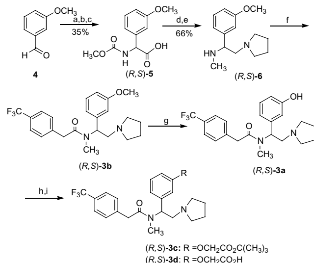
Scheme 1. Reagents and conditions: (a) NaCN, NH 4 Cl; (b) HCl (6 N), reflux; (c) methyl chloroformate, NaOH (1 N); (d) HOBT/DCC, pyrrolidine; (e) LAH, THF; (f) 4-trifluoromethylphenyl acetic acid, HOBT/DCC, CH 2 Cl 2 ; (g) BBr 3 , CH 2 Cl 2 , −70 °C; (h) t -butyl bromoacetate, K 2 CO 3 , DMF; (i) HCl (6 N), 95–100 °C.
